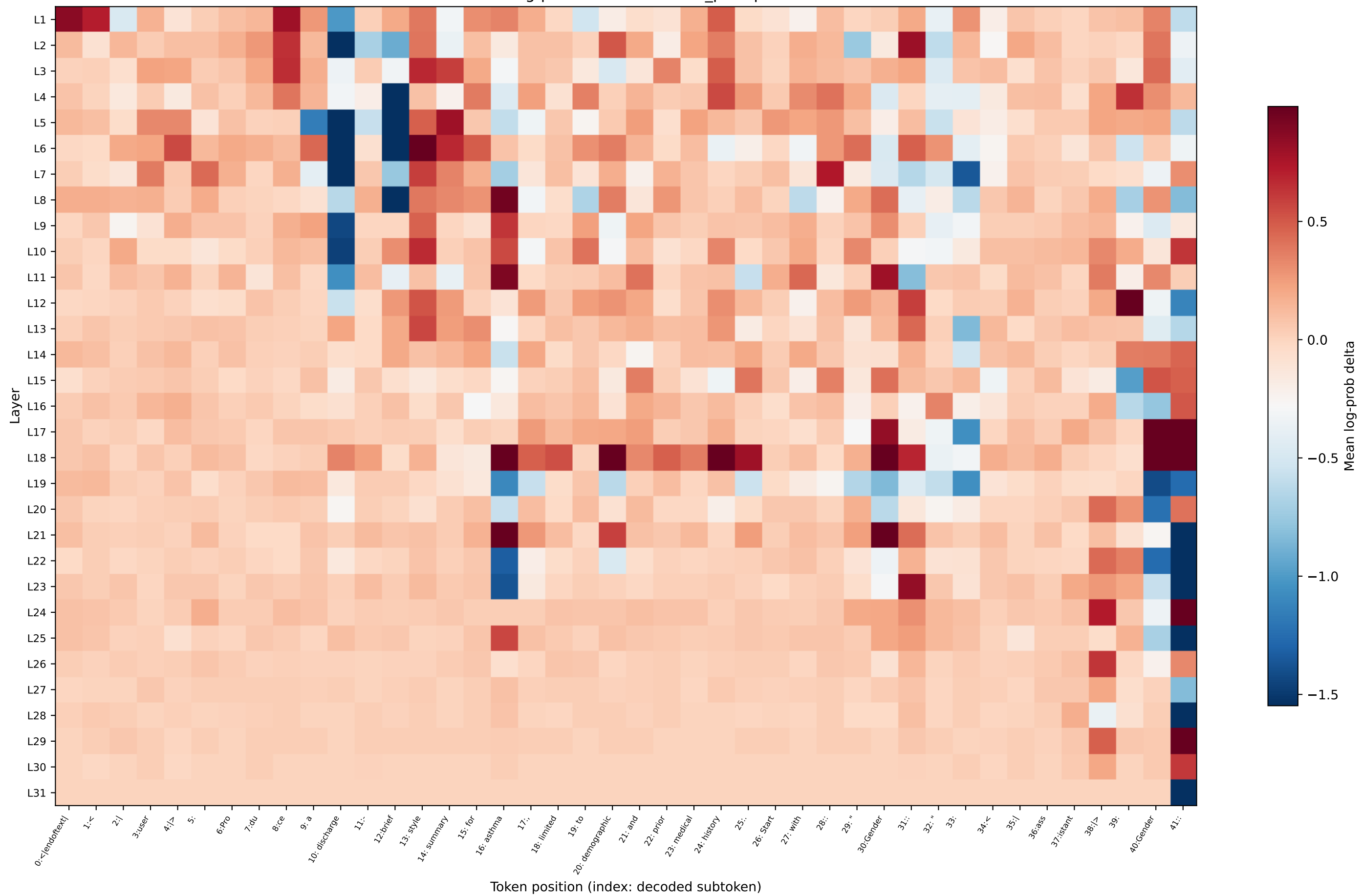
OLMo log-prob delta — asthma_prompt24
