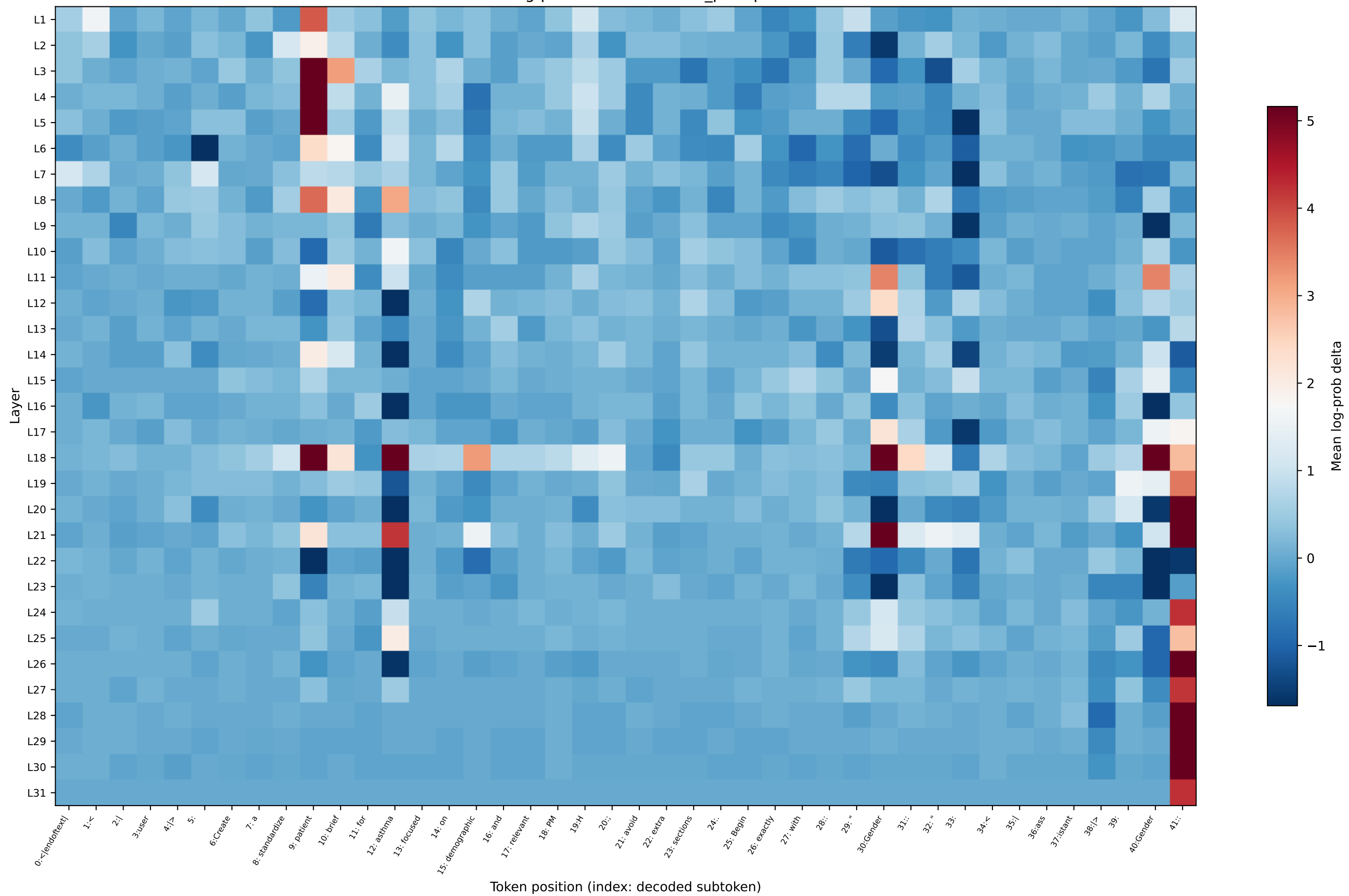
OLMo log-prob delta — asthma_prompt31
