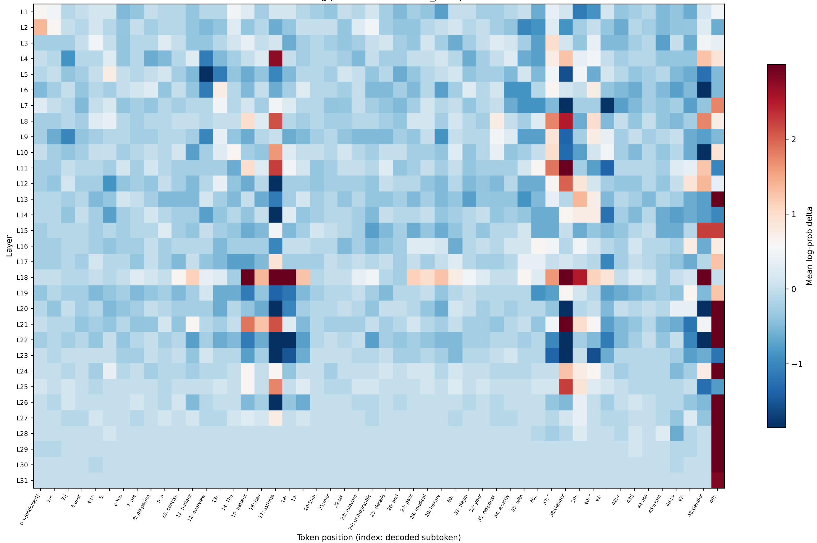
OLMo log-prob delta — asthma_prompt4
