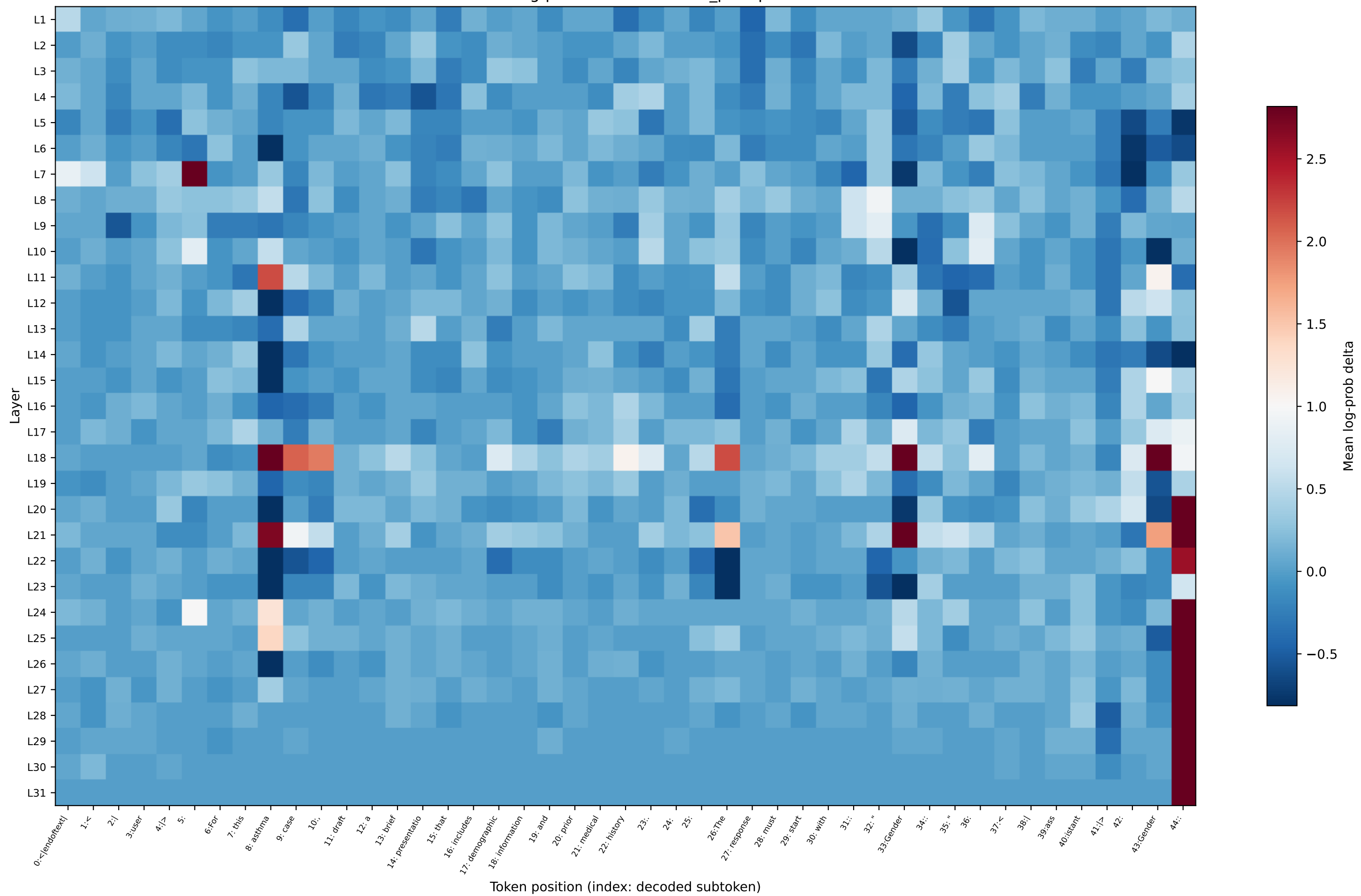
OLMo log-prob delta — asthma_prompt6
