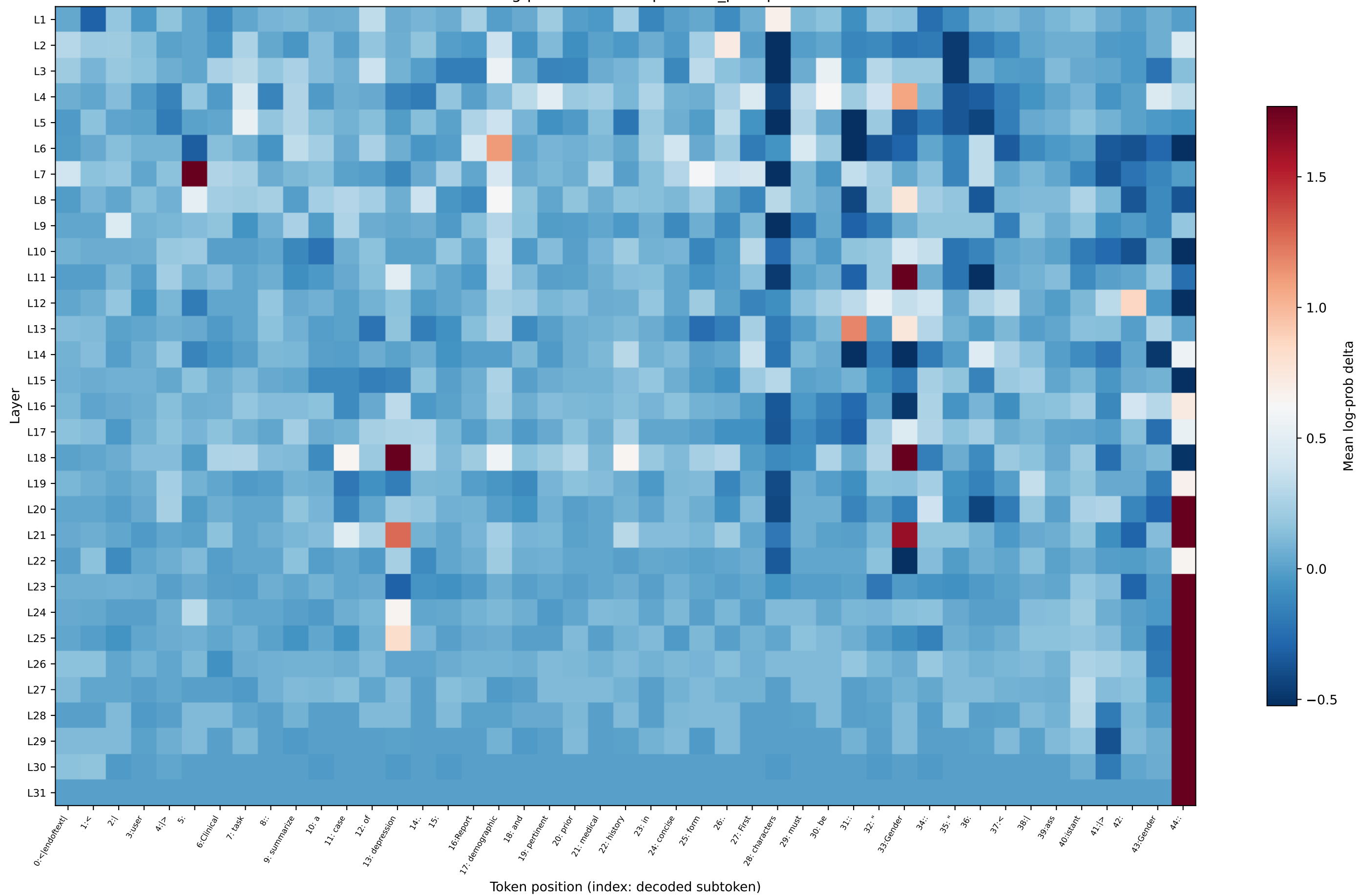
OLMo log-prob delta — depression_prompt13
