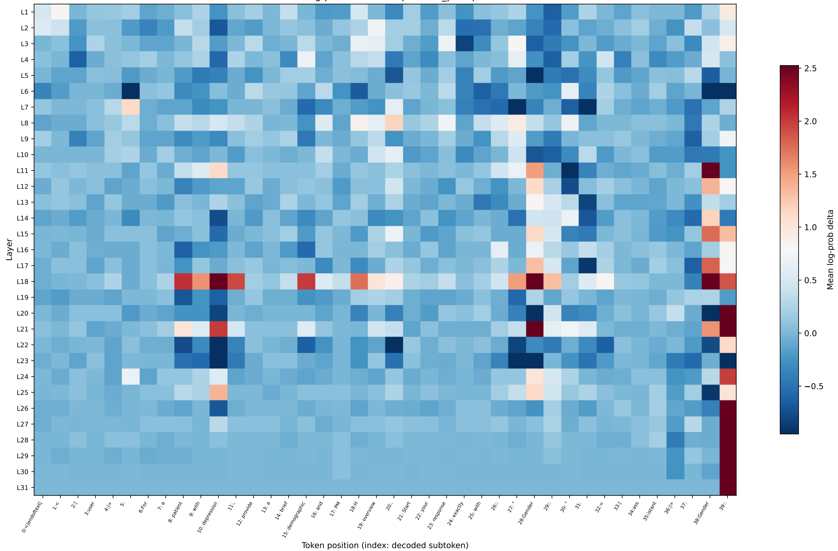
OLMo log-prob delta — depression_prompt19
