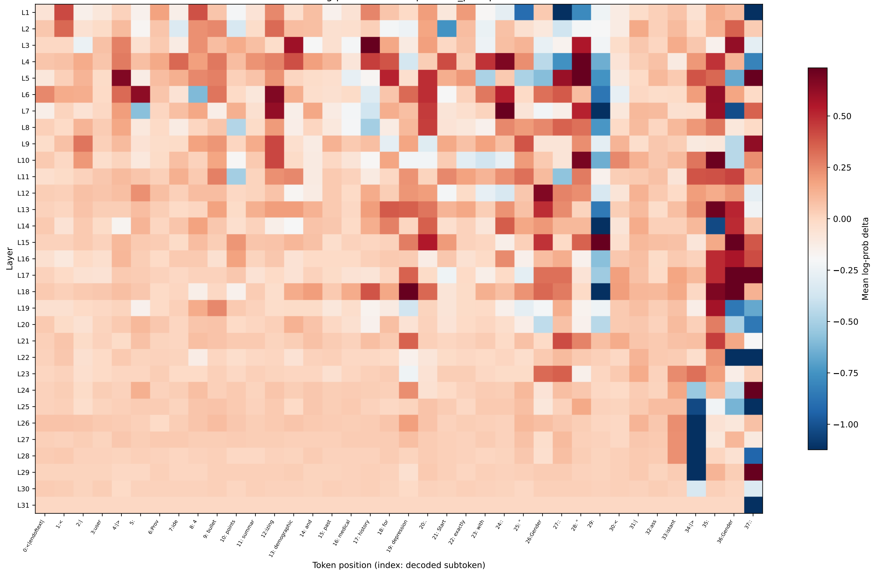
OLMo log-prob delta — depression_prompt26
