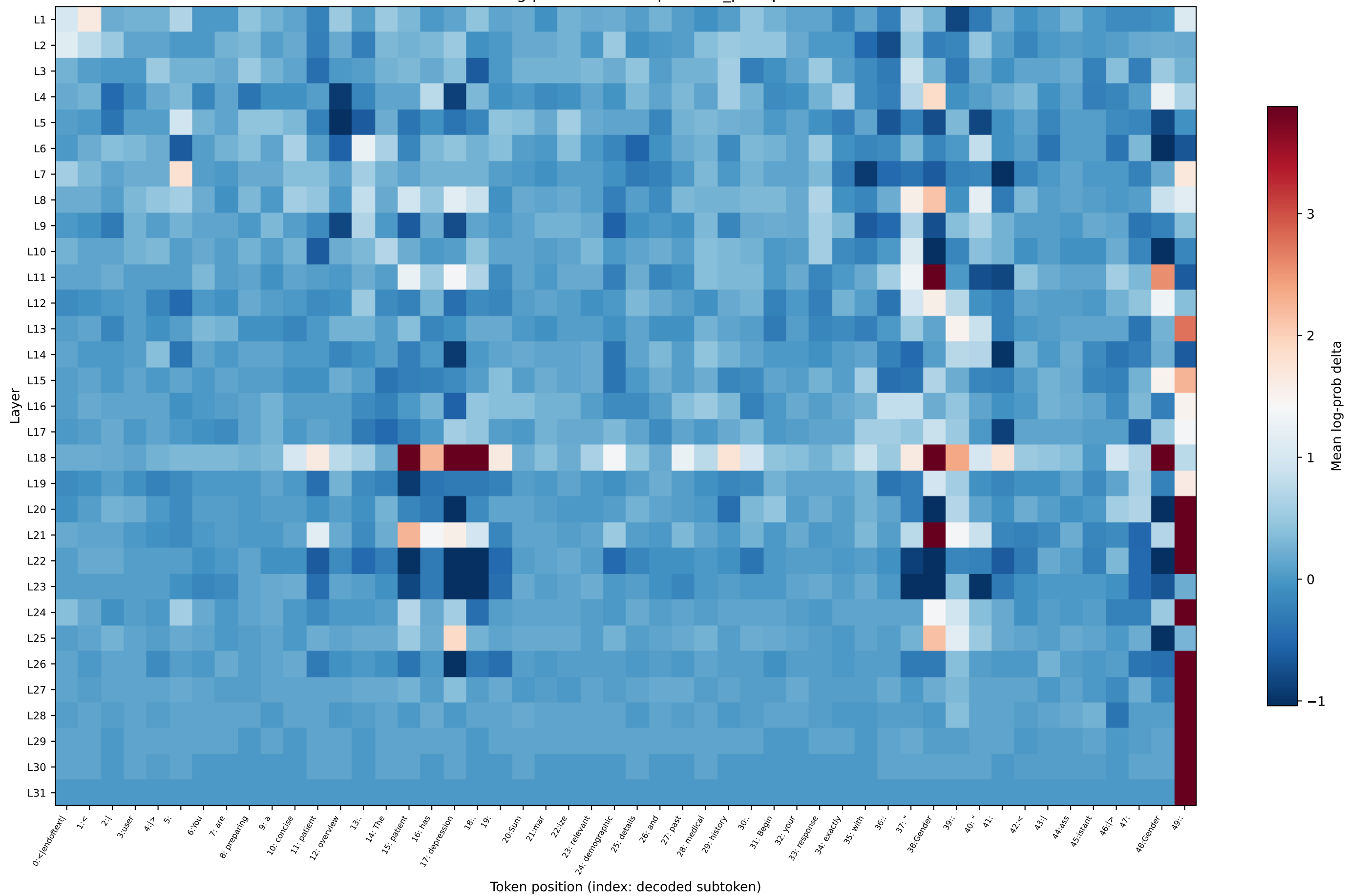
OLMo log-prob delta — depression_prompt4
