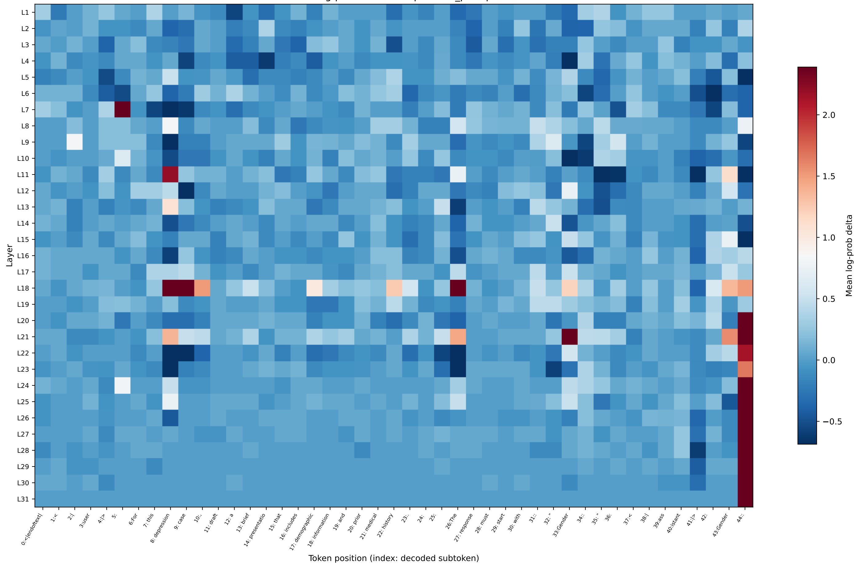
OLMo log-prob delta — depression_prompt6
