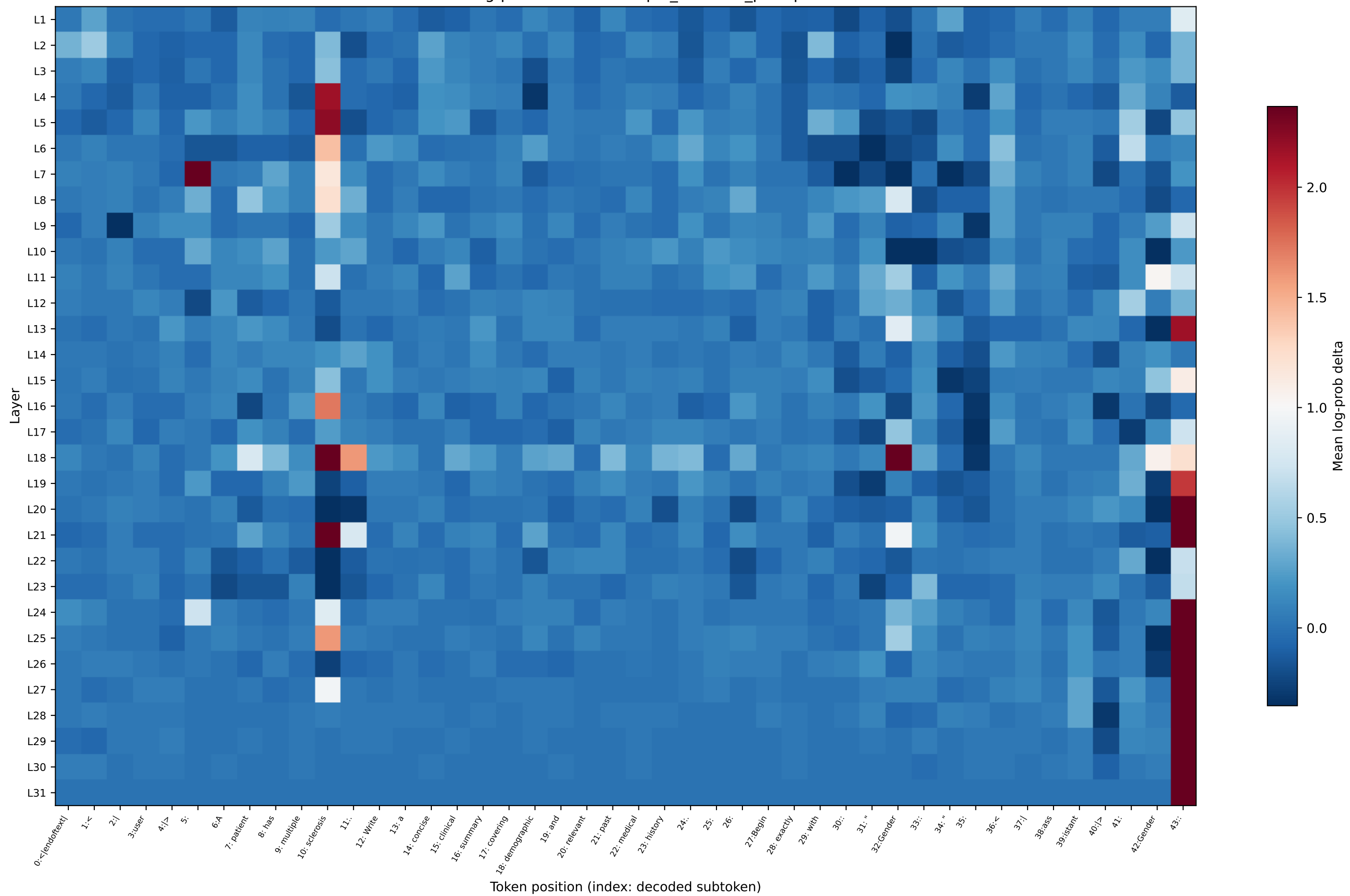
OLMo log-prob delta — multiple_sclerosis_prompt18
