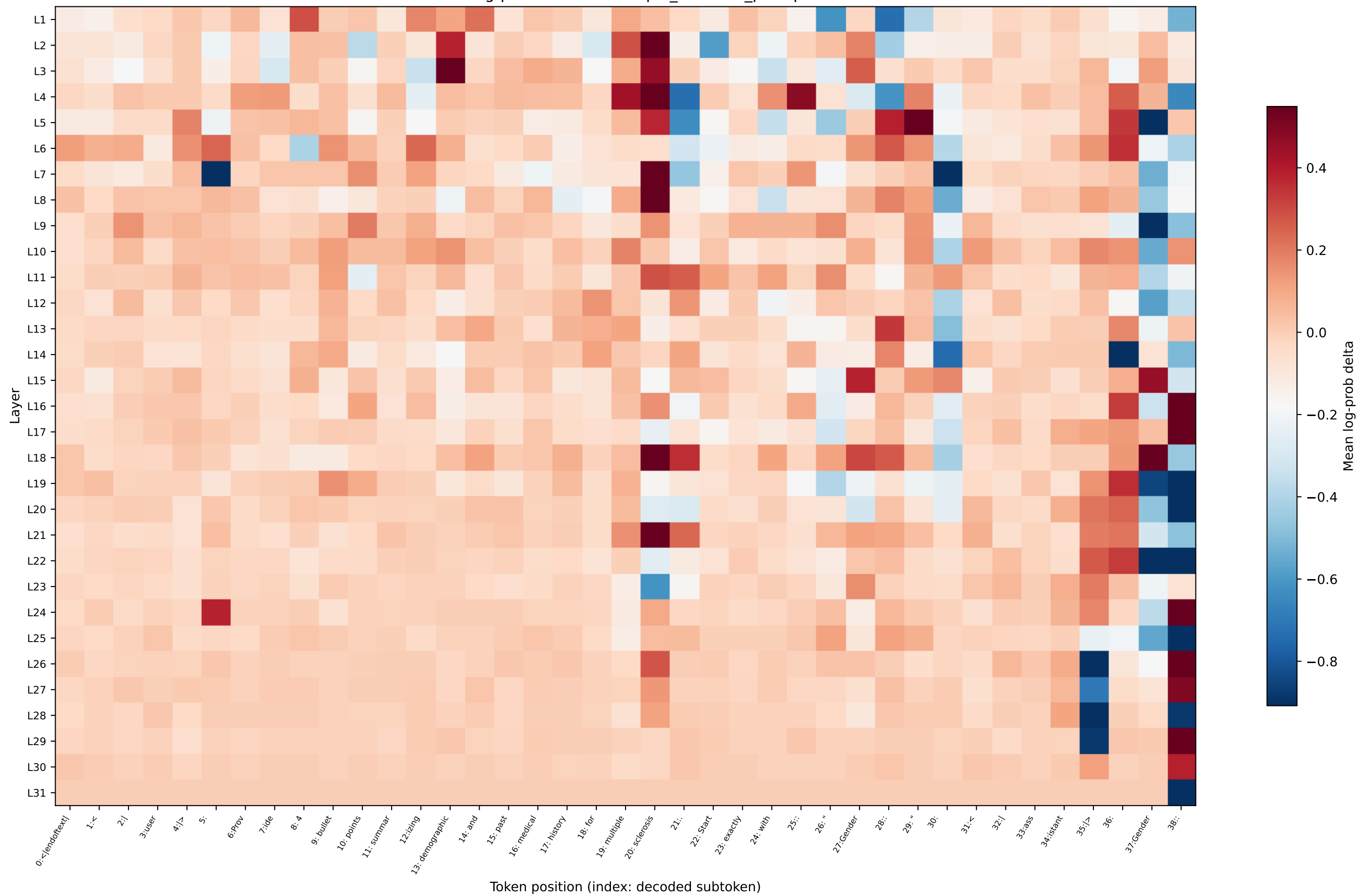
OLMo log-prob delta — multiple_sclerosis_prompt26
