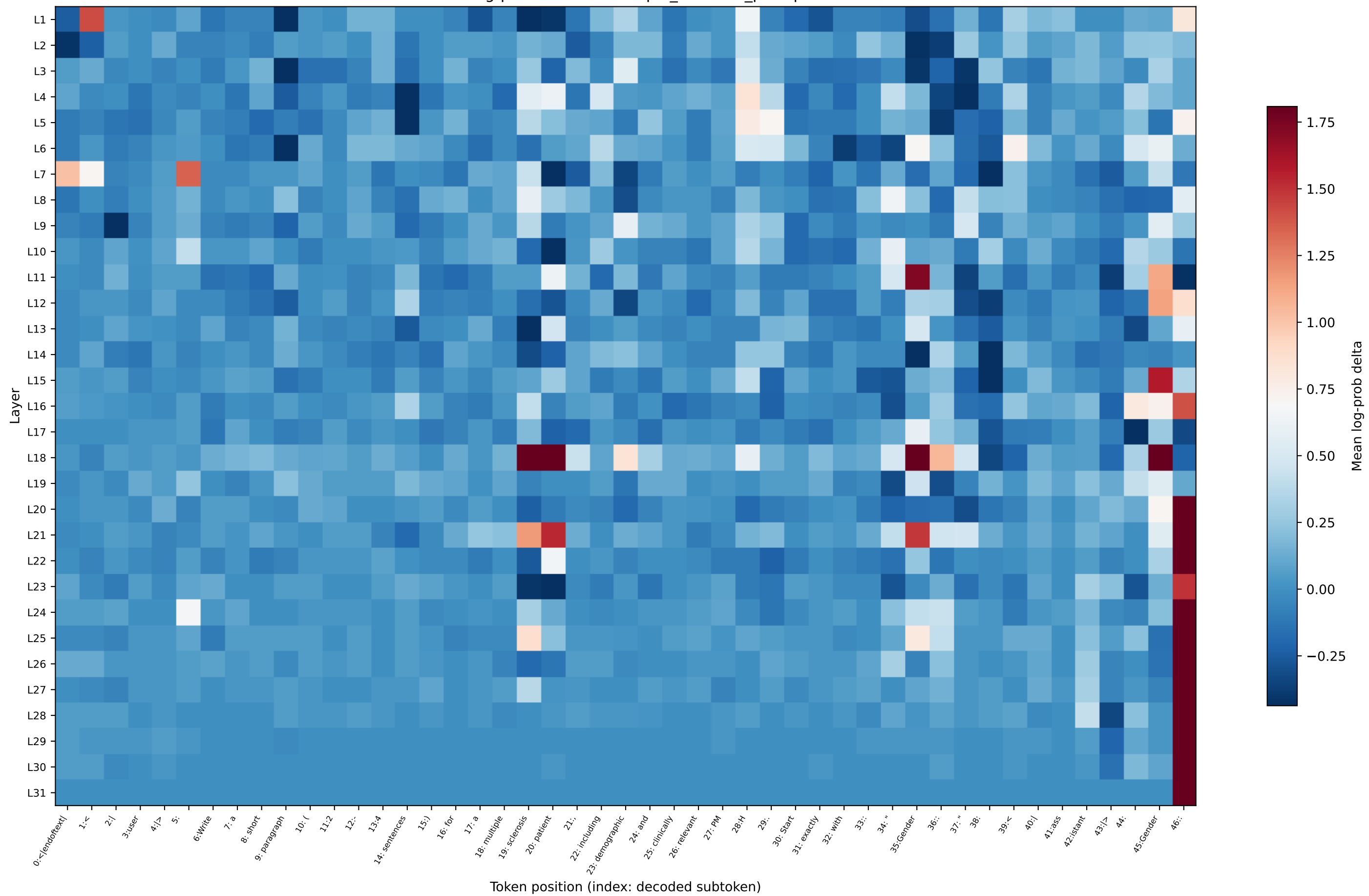
OLMo log-prob delta — multiple_sclerosis_prompt29
