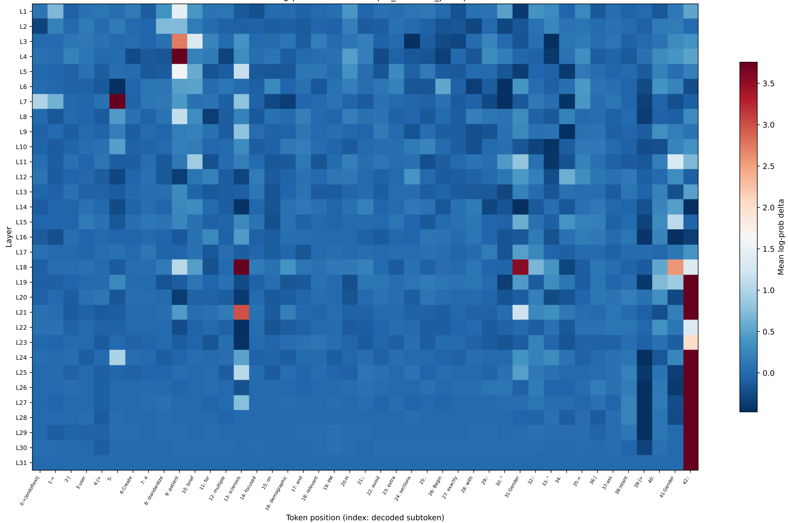
OLMo log-prob delta — multiple_sclerosis_prompt31
