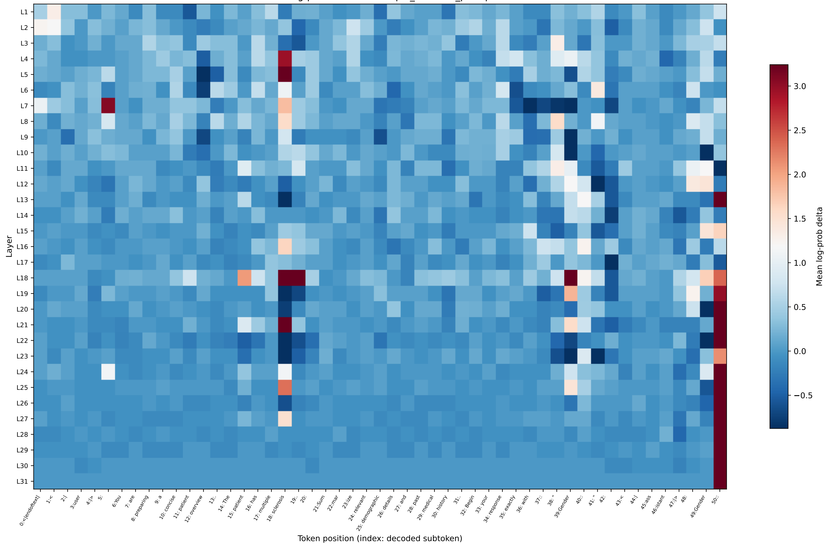
OLMo log-prob delta — multiple_sclerosis_prompt4
