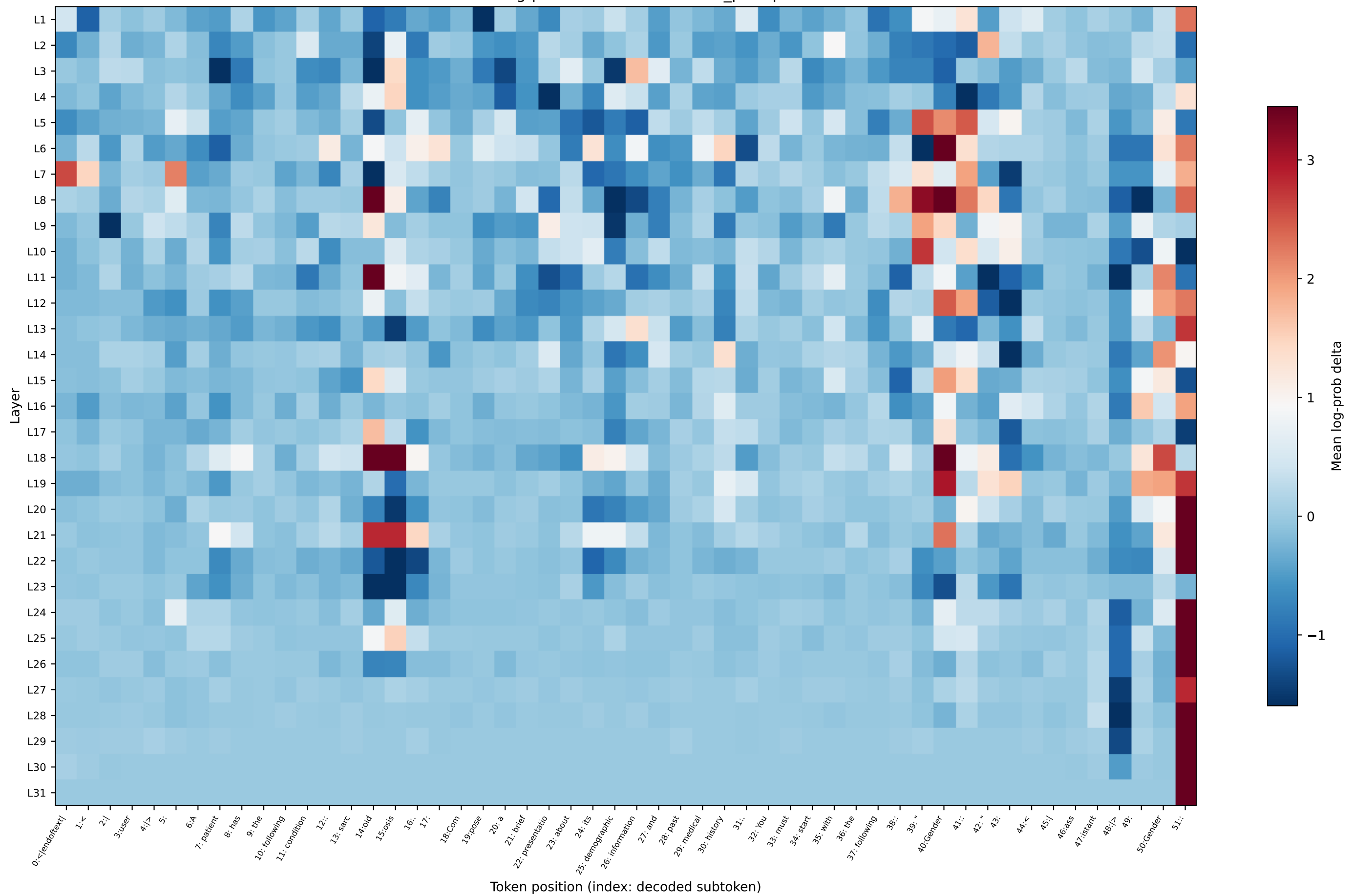
OLMo log-prob delta — sarcoidosis_prompt1
