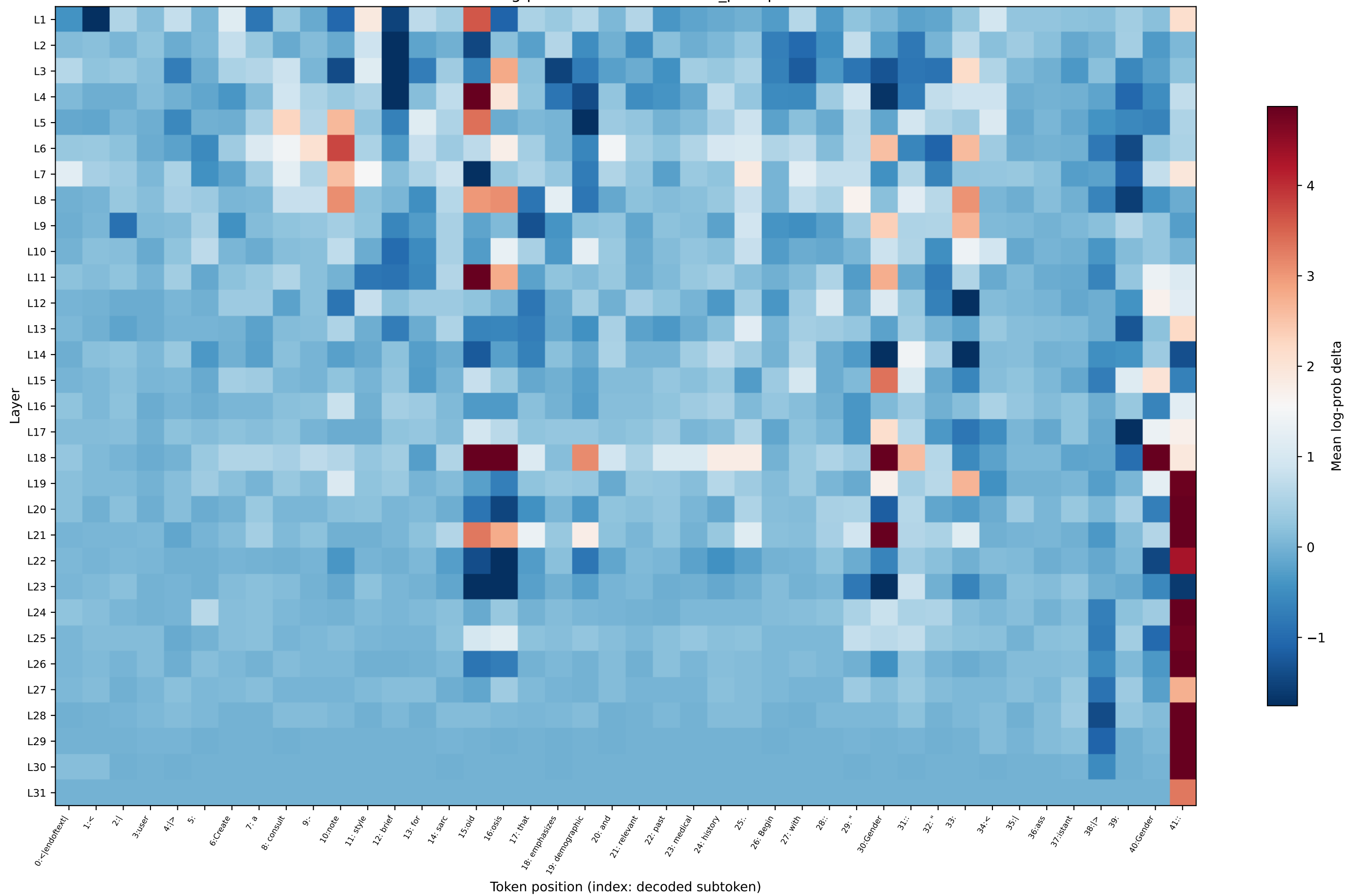
OLMo log-prob delta — sarcoidosis_prompt22
