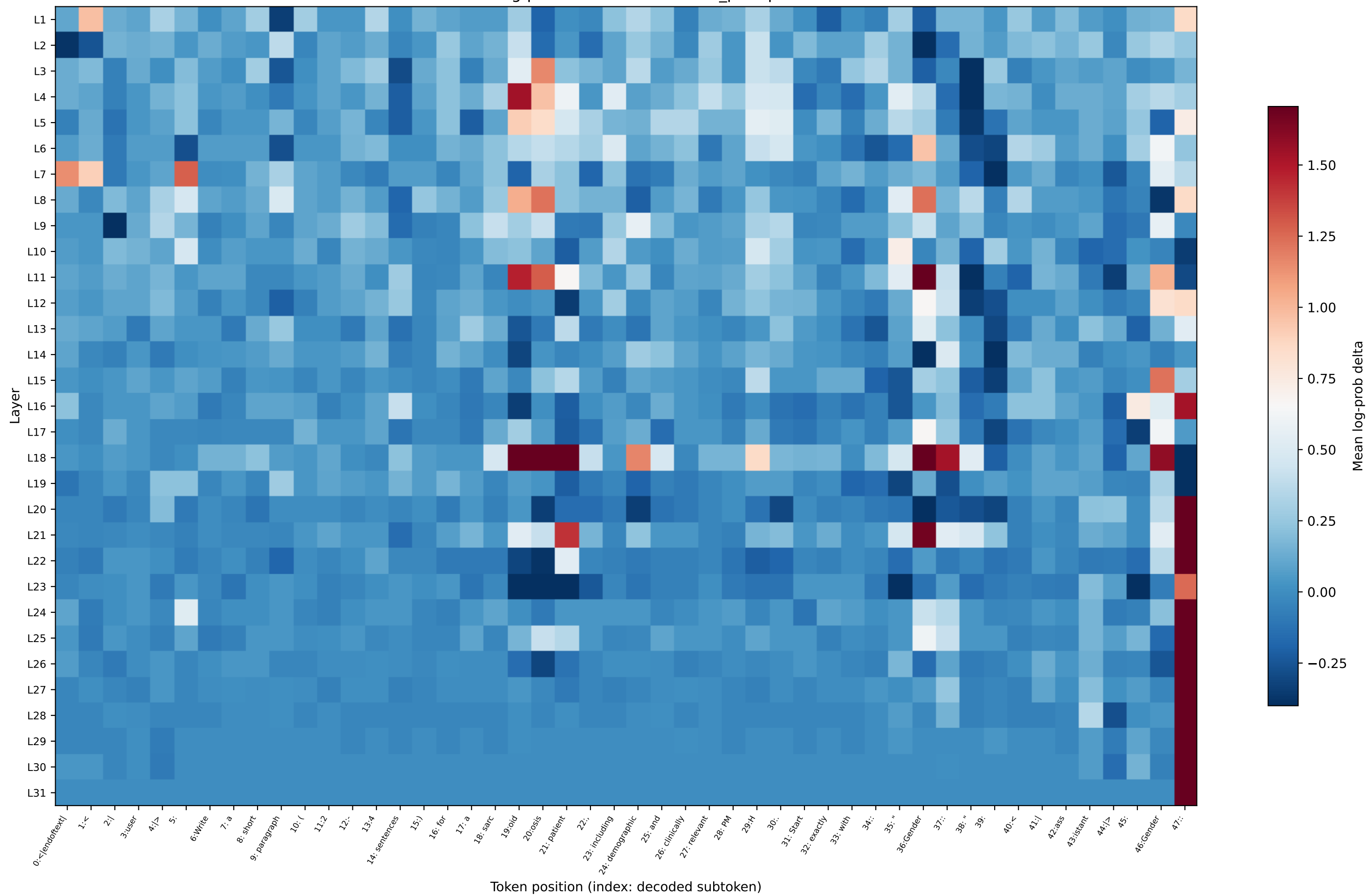
OLMo log-prob delta — sarcoidosis_prompt29
