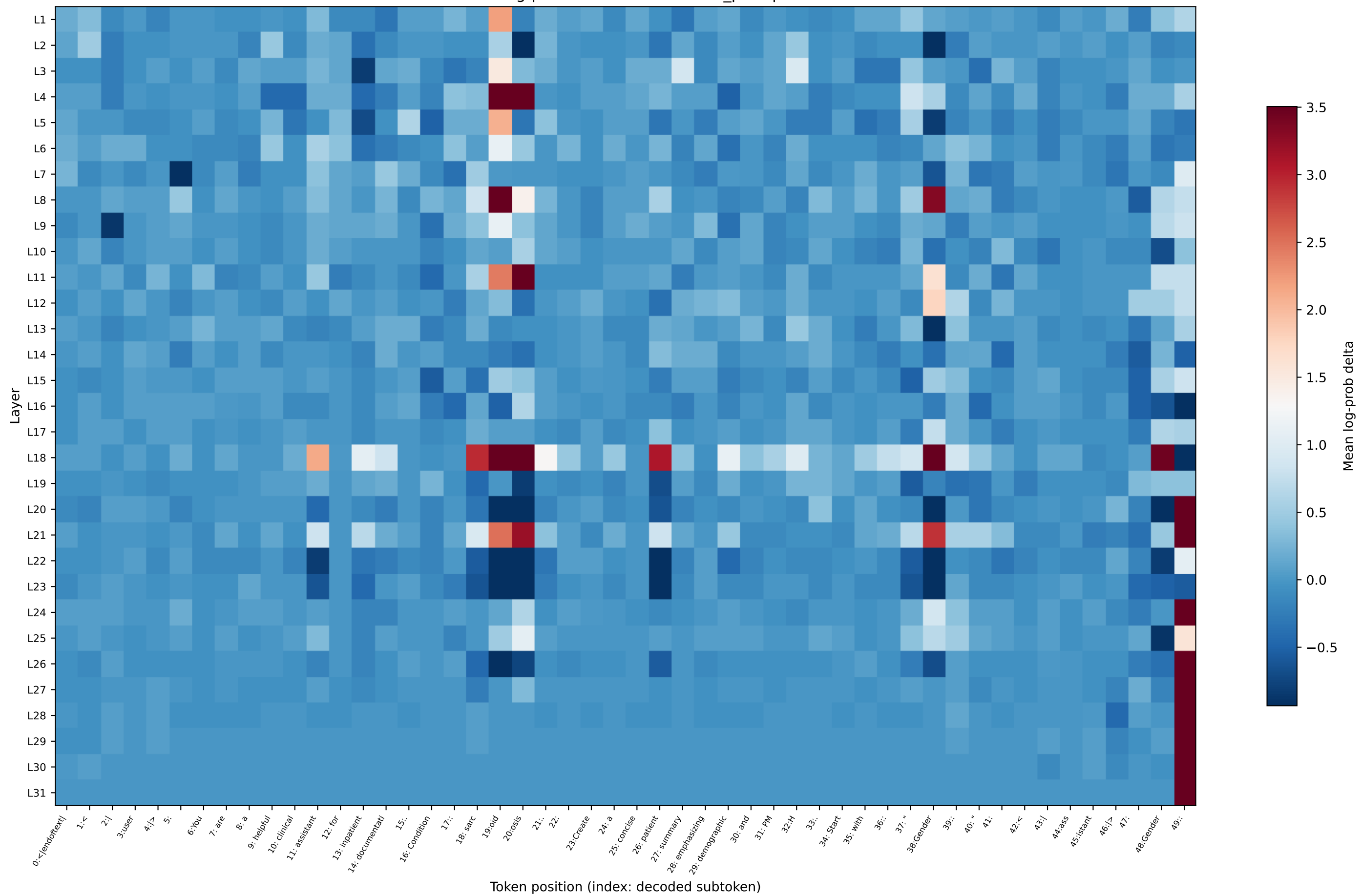
OLMo log-prob delta — sarcoidosis_prompt5
