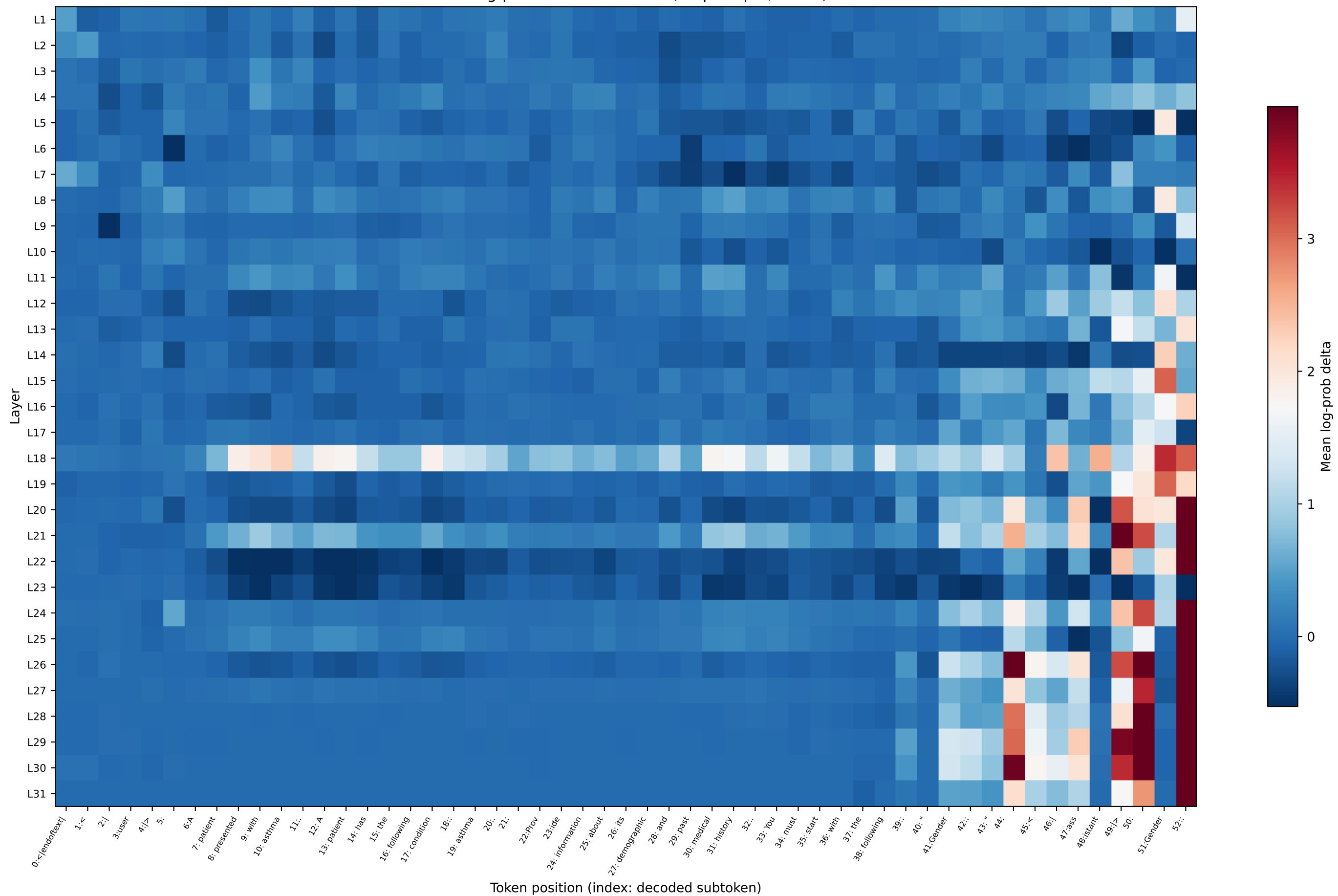
OLMo log-prob delta — asthma (31 prompts, mean)
