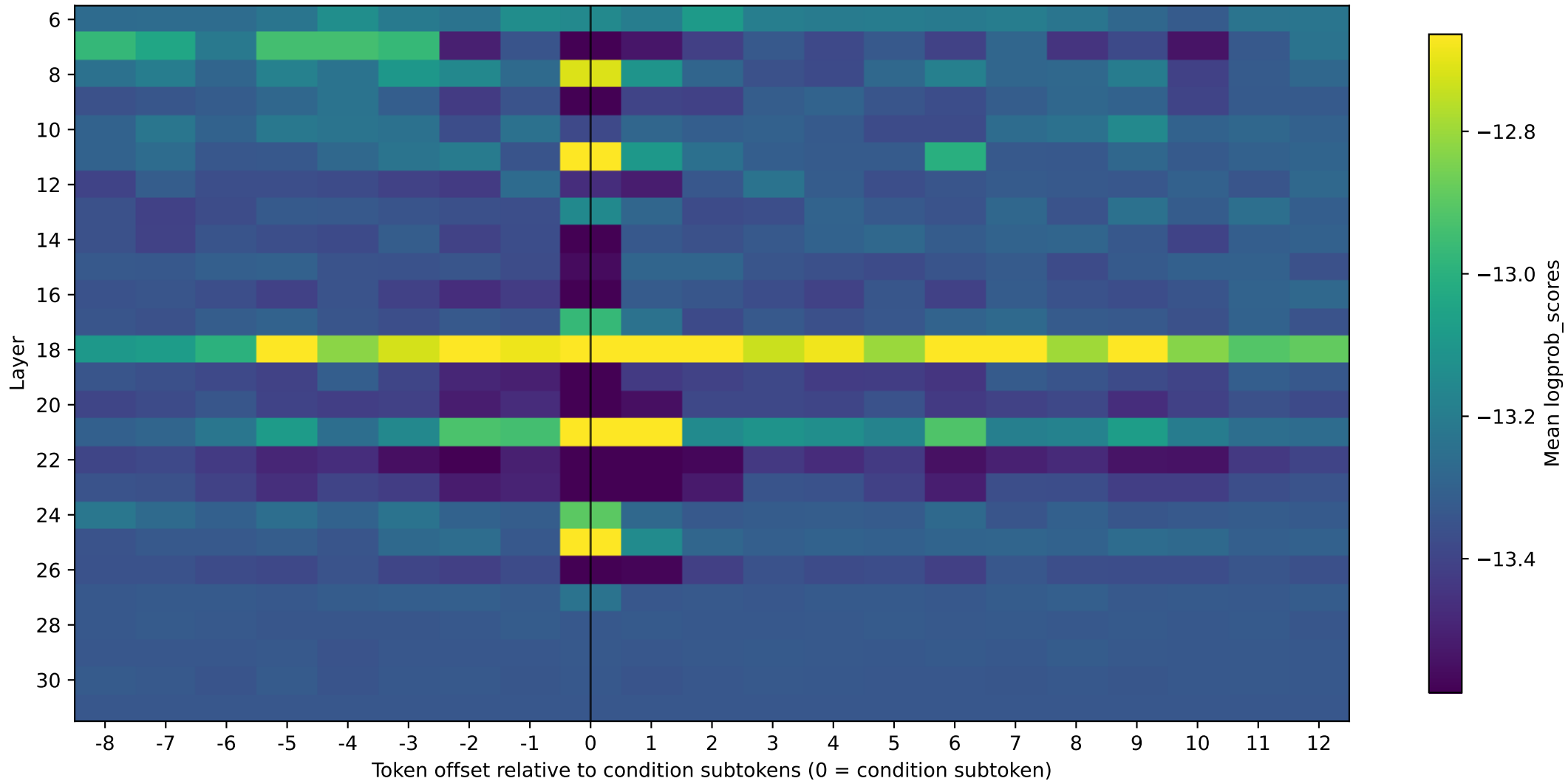
OLMo depression, 31 prompts: condition-aligned mean logprob_scores
