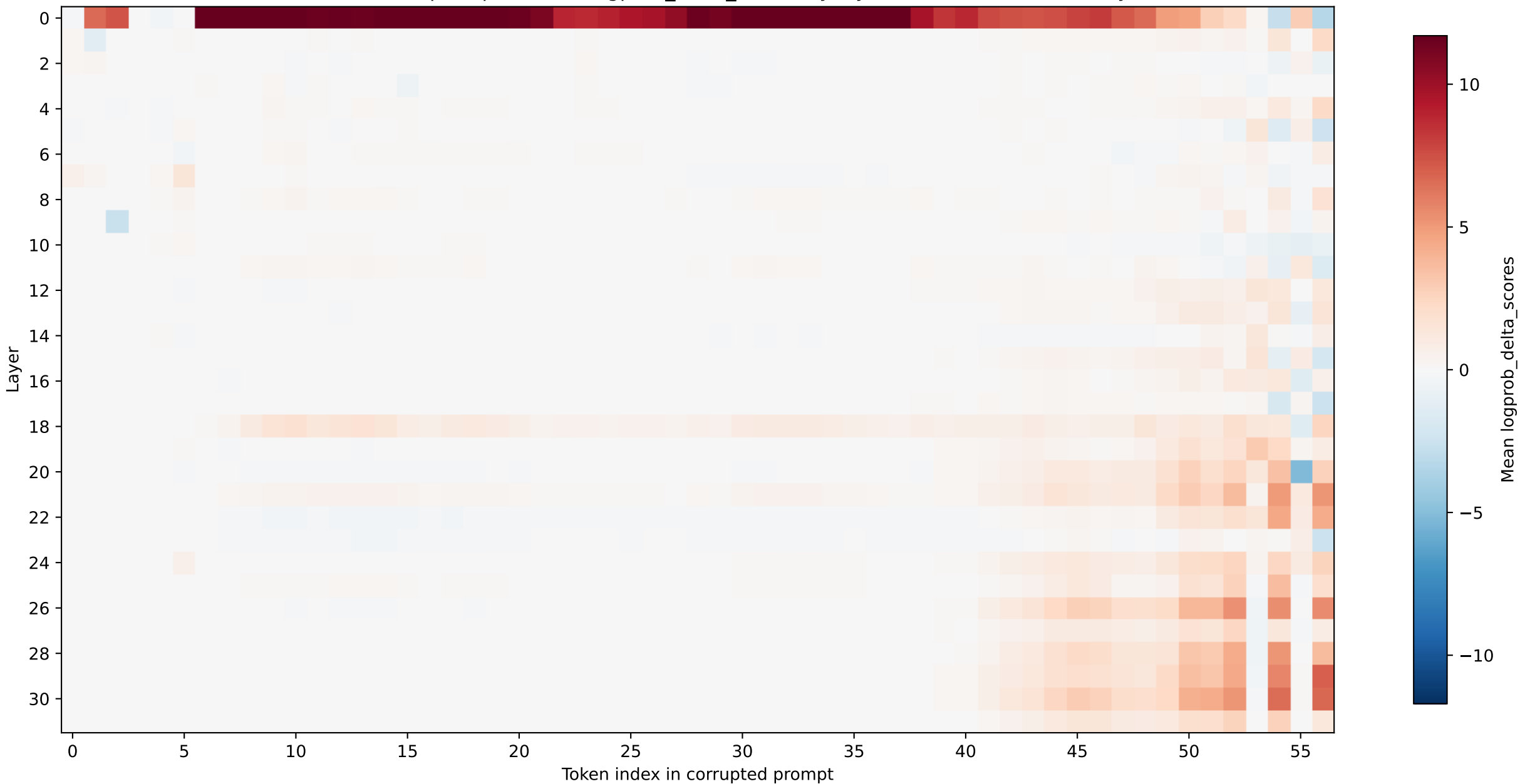
OLMo all conditions/prompts: mean logprob_delta_scores by layer and token index (all layers)
