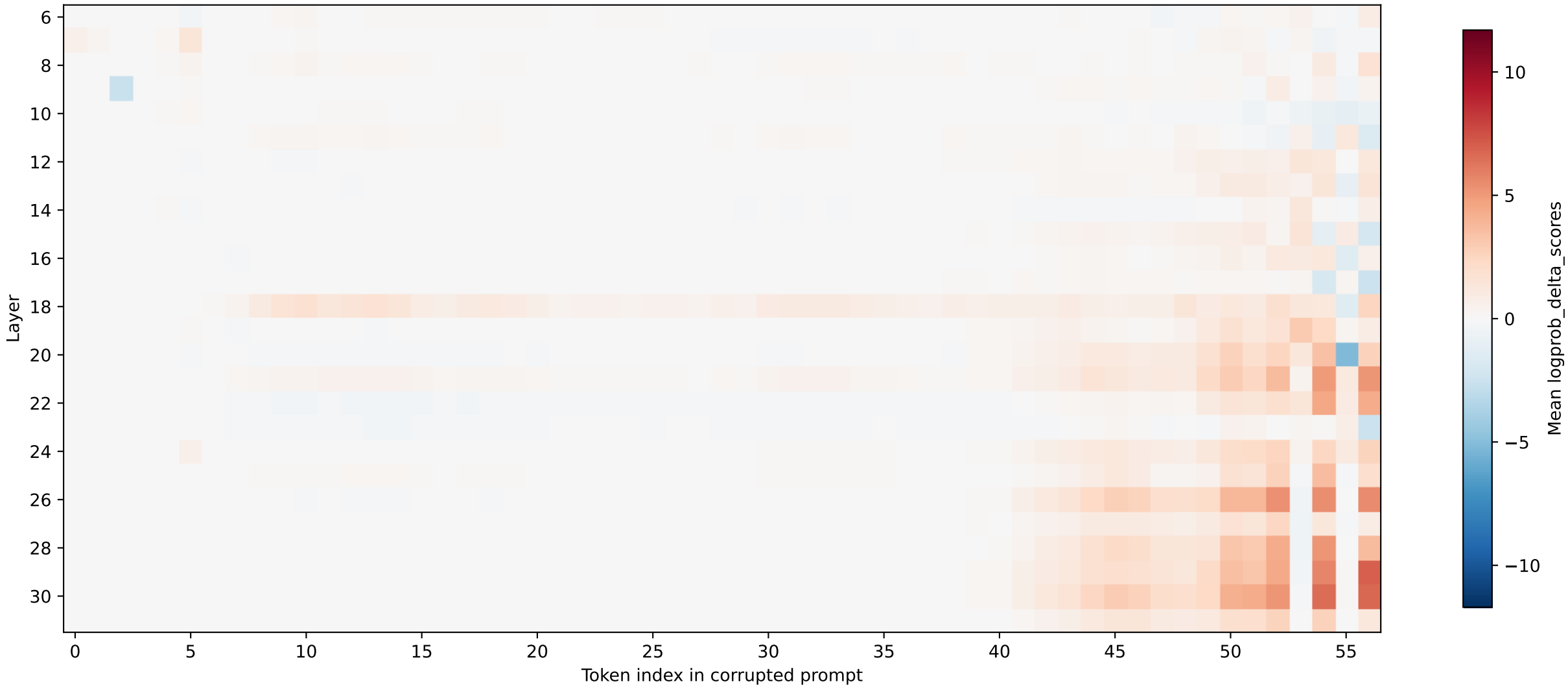
OLMo all conditions/prompts: mean logprob_delta_scores by layer and token index (layers 6 plus)
