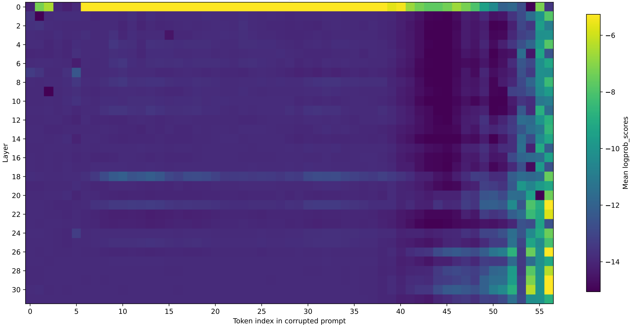
OLMo all conditions/prompts: mean logprob_scores by layer and token index (all layers)
