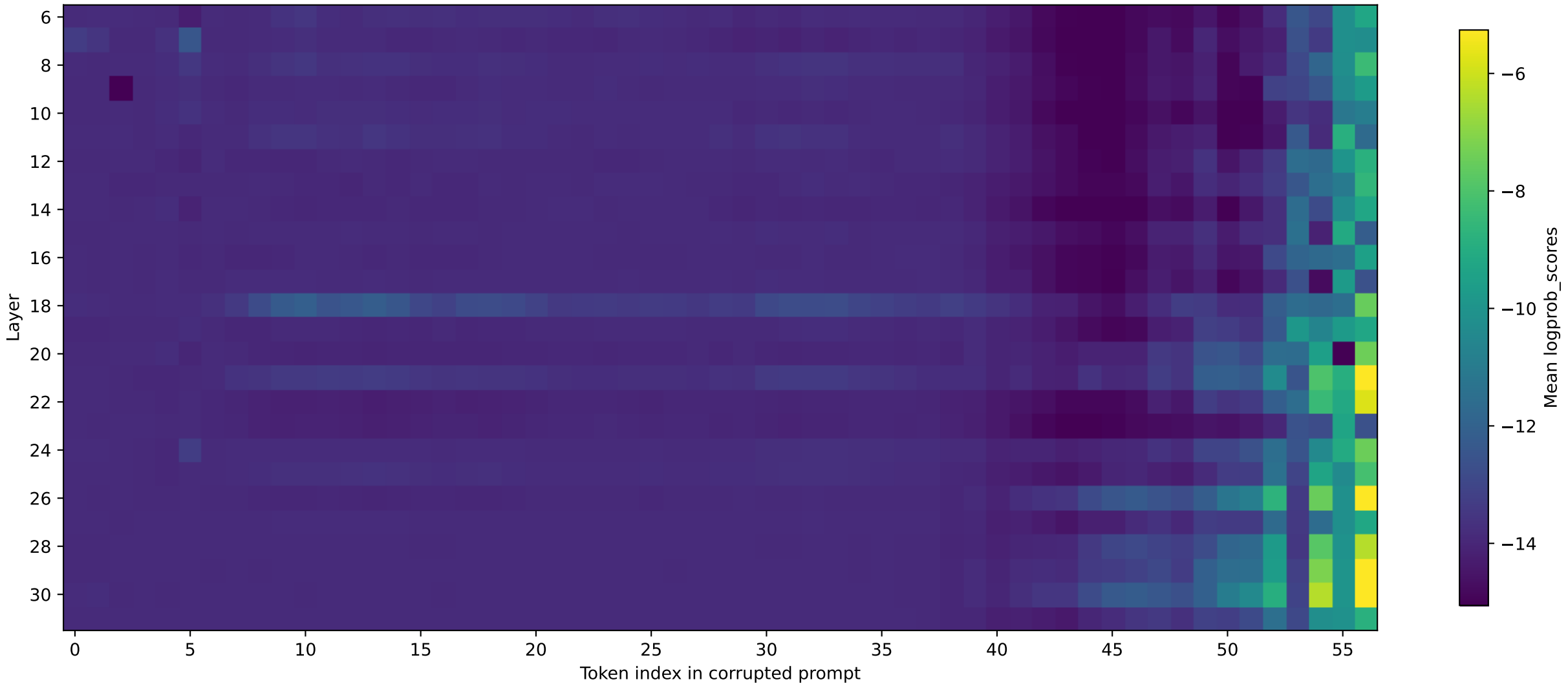
OLMo all conditions/prompts: mean logprob_scores by layer and token index (layers 6 plus)
