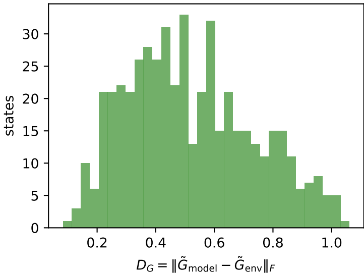
Trace-normalized metric discrepancy
