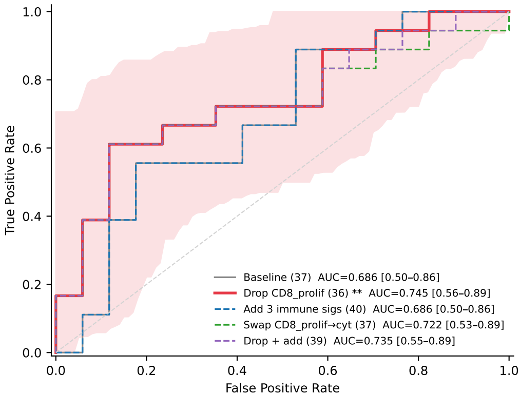
Nested outer-LOOCV ROC — ElasticNet (N=35) immune-feature ablation
