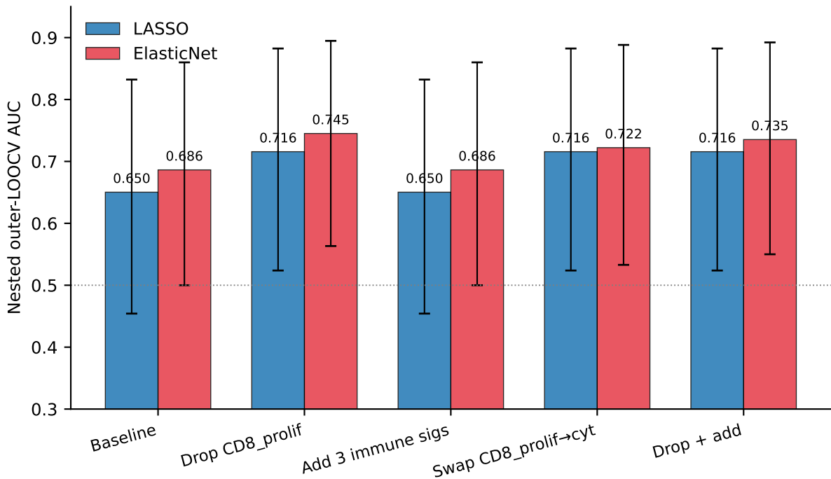
AUC across feature-set ablations (95% bootstrap CI, n=2000)
