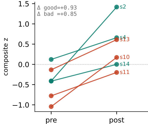
P2 TLS-8
