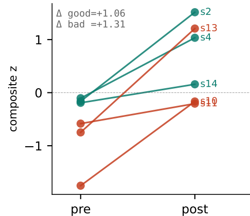
P4 GC-TF
