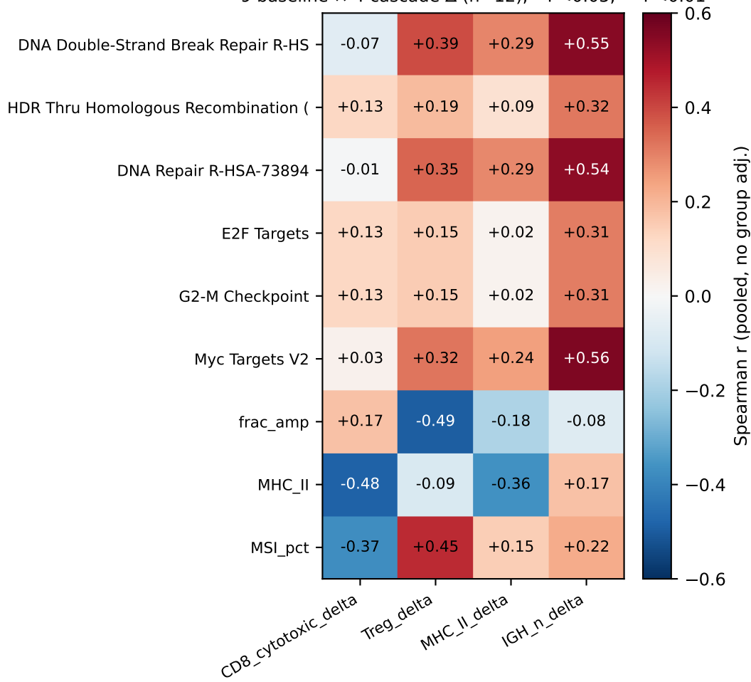
Configuration A: pooled Spearman, no group adjustment 9 baseline x 4 cascade \Delta (n=12), * P<0.05, ** P<0.01
