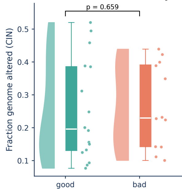
Chromosomal instability
