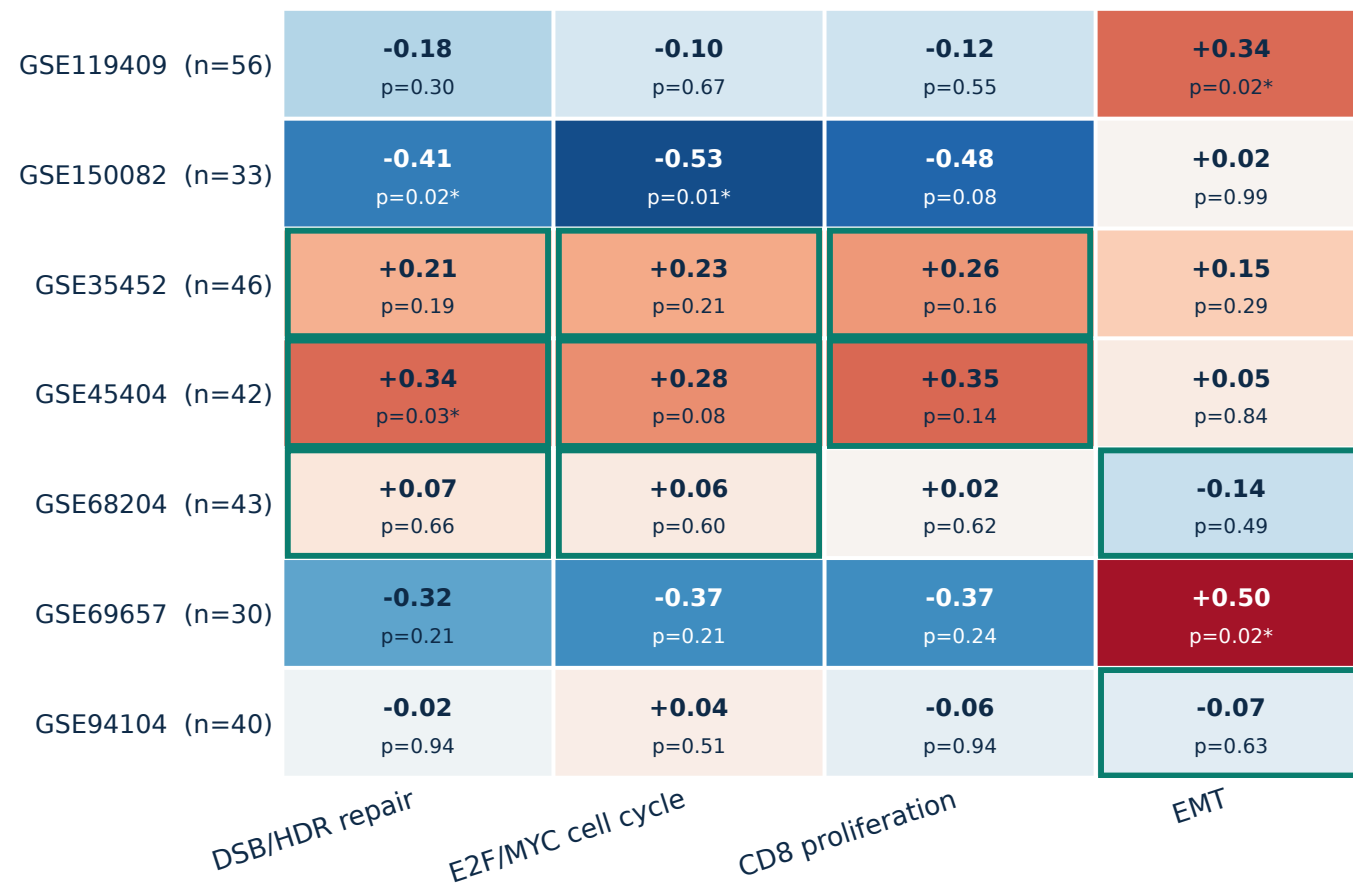
B Cohort × signature effect size
