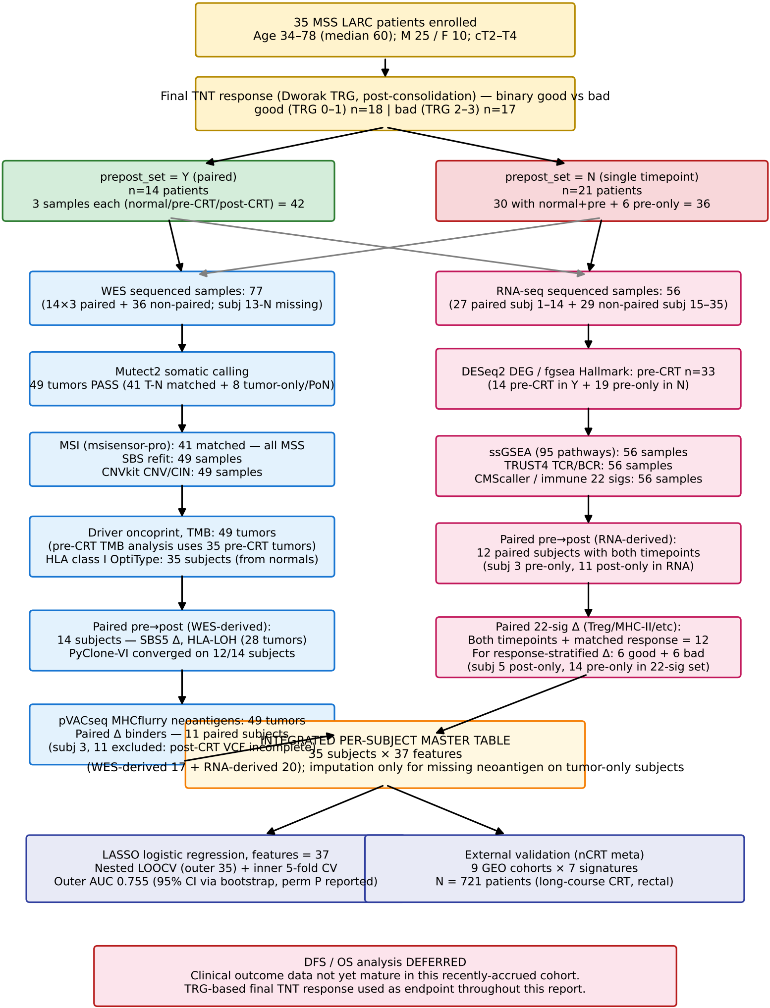
Fig S1. CONSORT-style sample flow diagram reconciling all per-analysis sample counts. WES branch (blue) includes 77 sequenced samples collapsing to 49 PASS tumor somatic VCFs; RNA-seq branch (pink) includes 56 samples collapsing to 33 pre-CRT for DEG/GSEA and 12 paired pre/post for Δ analysis; integration produces a 35x37 subject-level master.
