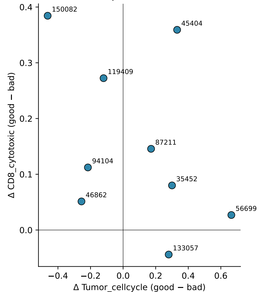
CD8 effector vs tumor proliferation decouple across cohorts
