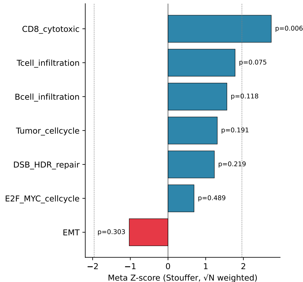
Signature-level meta-analysis (9 nCRT cohorts)
