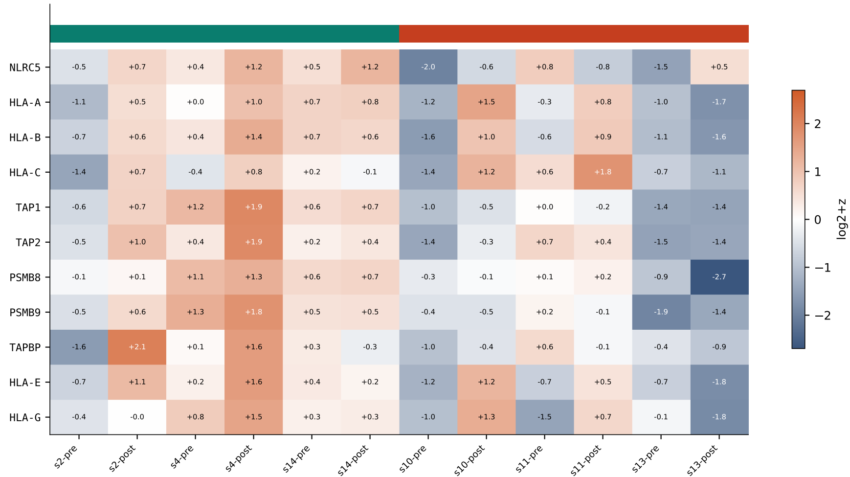
HLA class I antigen presentation machinery per subject × timepoint (log2+z)
