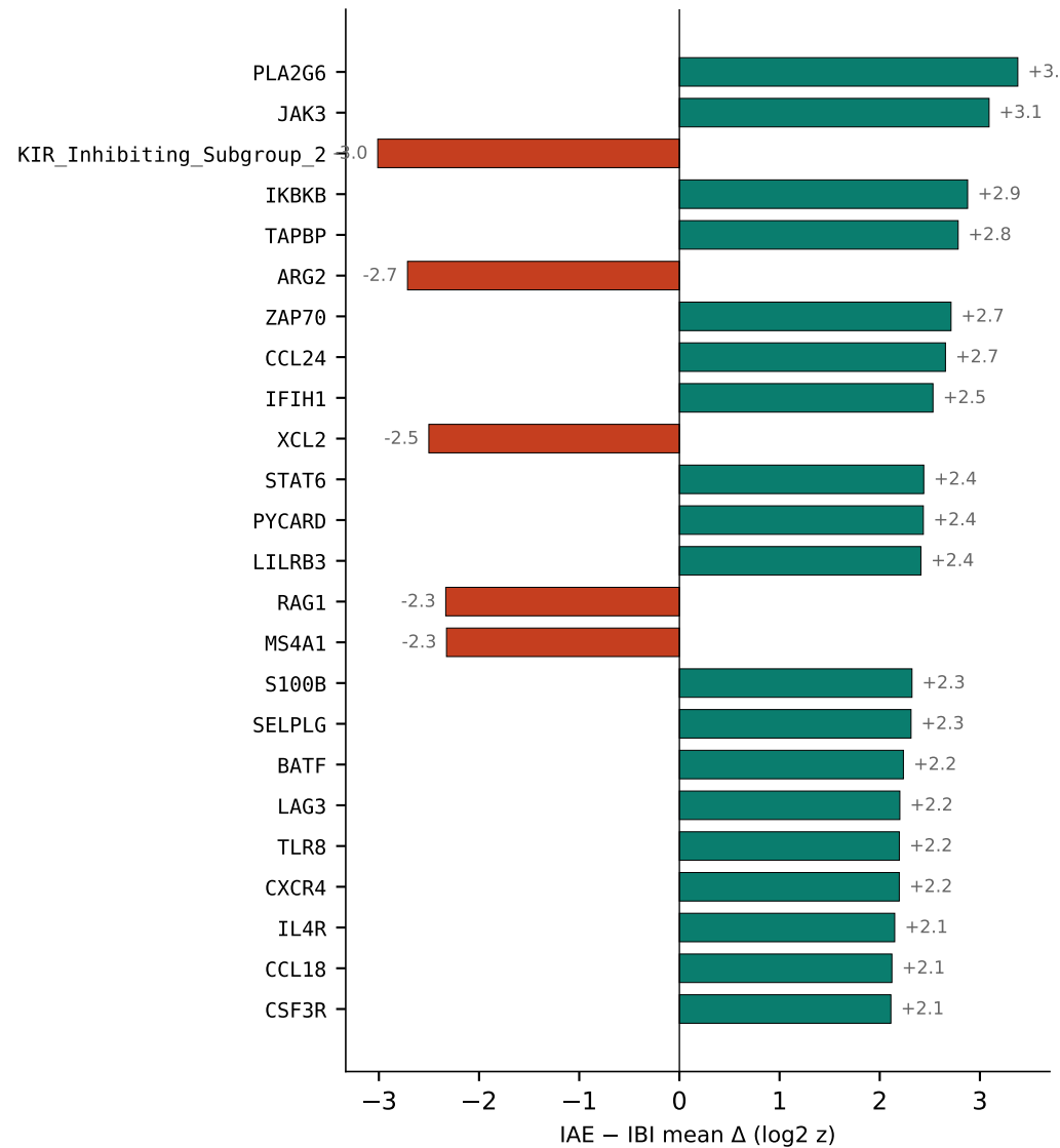
Gene level: top 24 by |IAE - IBI|
