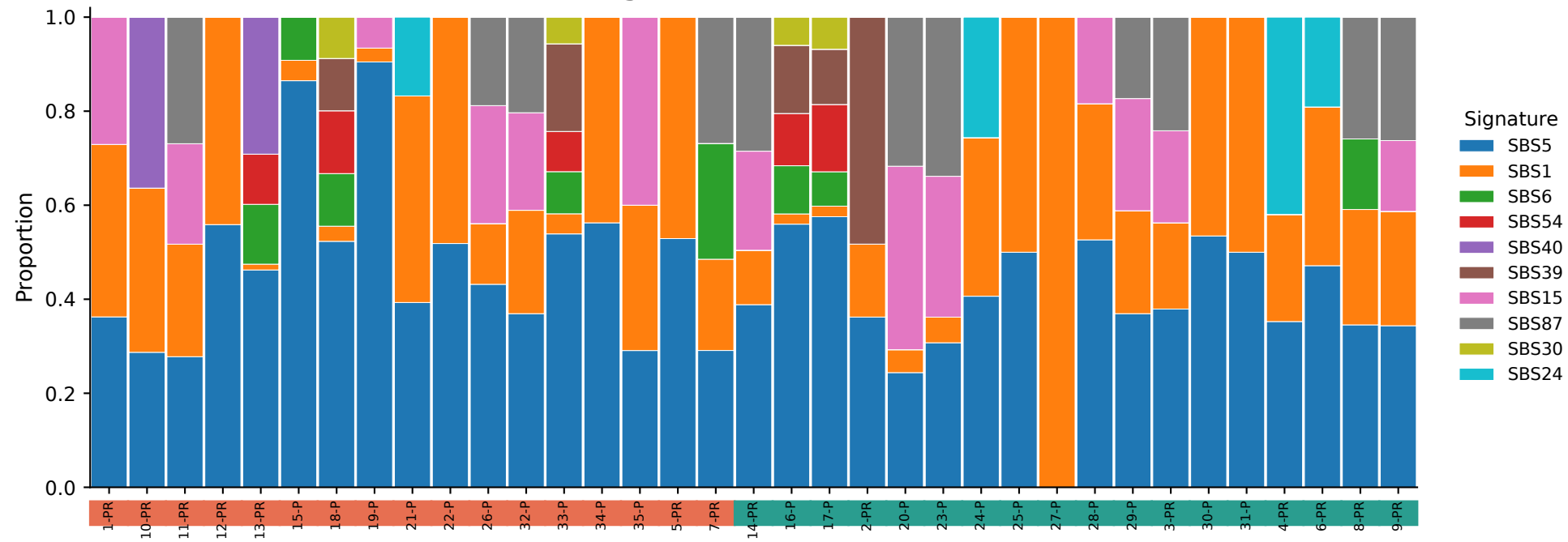
SBS mutational signature composition (pre-treatment)
