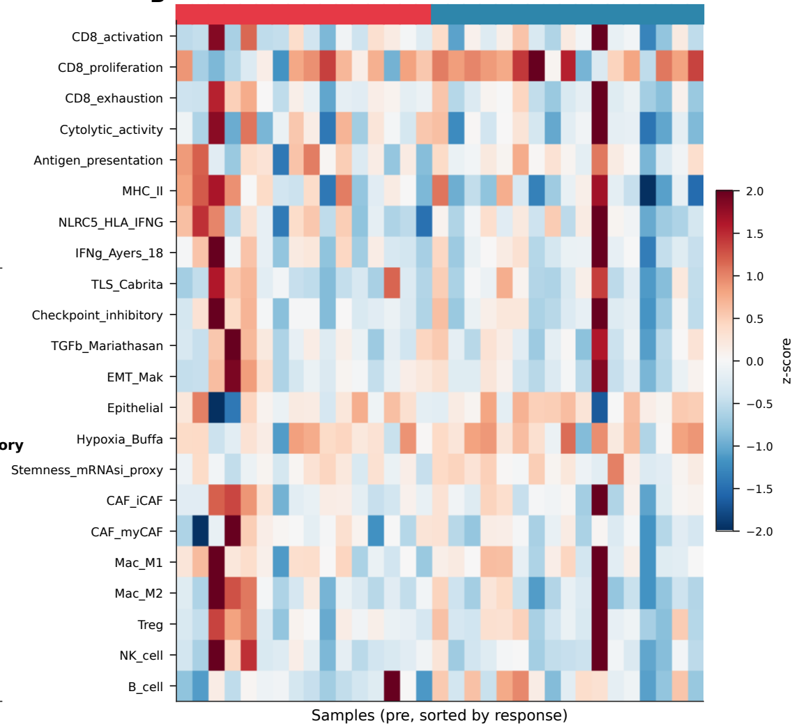
Figure 3. Pre-treatment immune and pathway signatures
