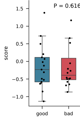
Figure 3. Pre-treatment immune and pathway signatures
