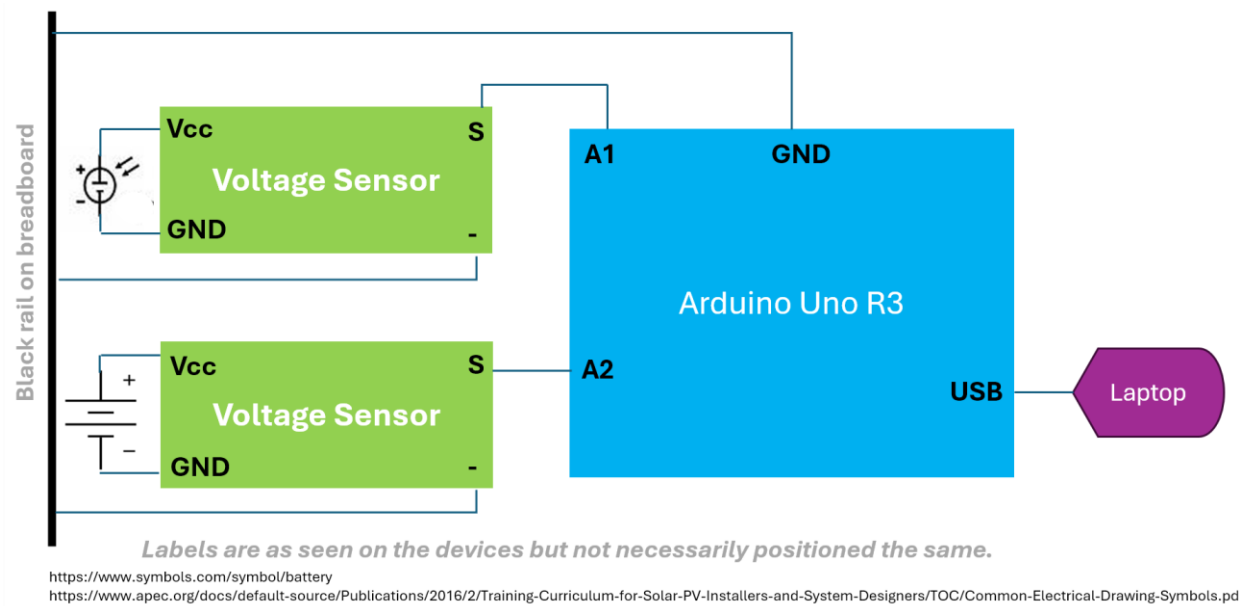
Figure 4. Circuit for solar system monitoring.
