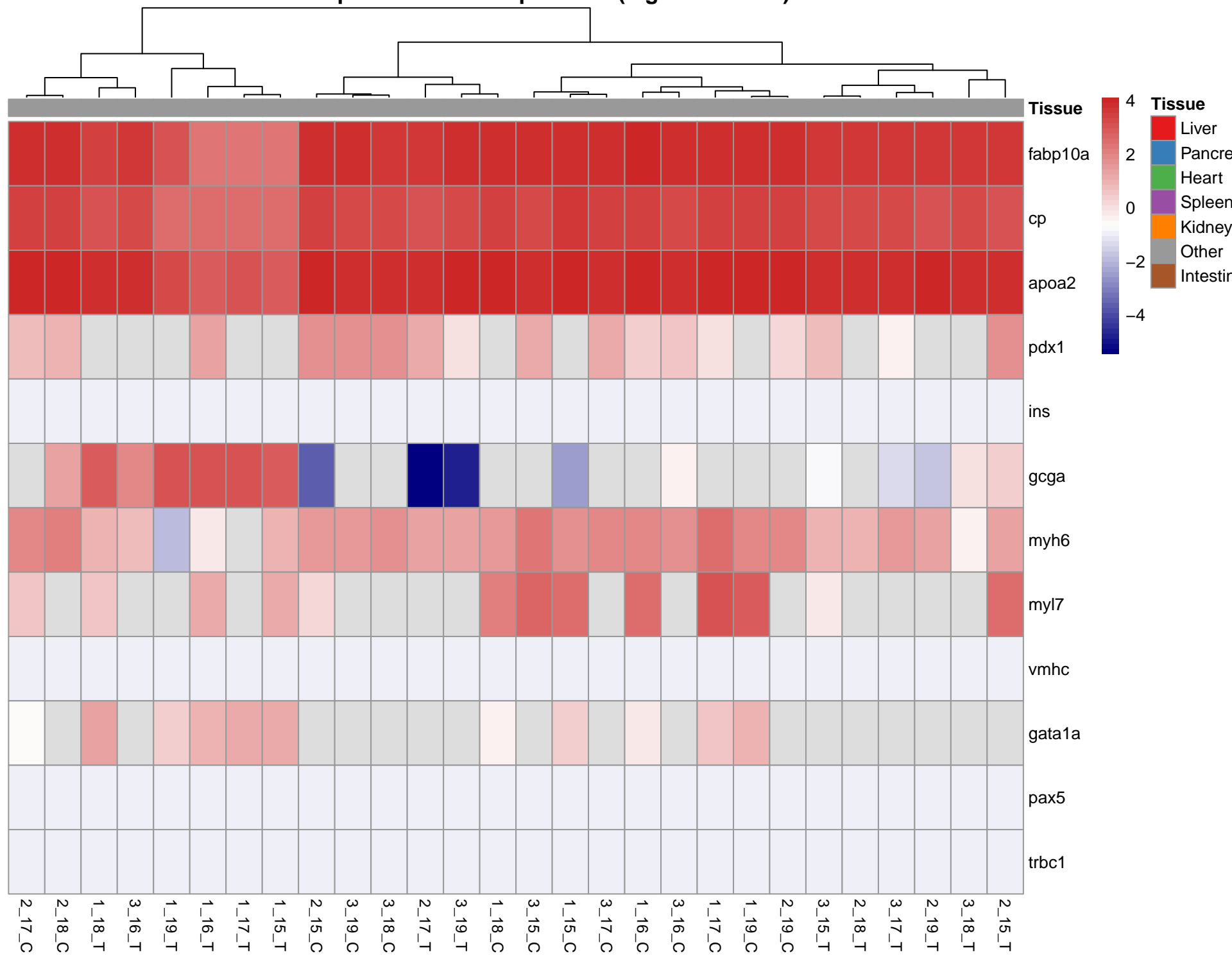
Tissue-specific marker expression (log2 CPM + 0.5)
