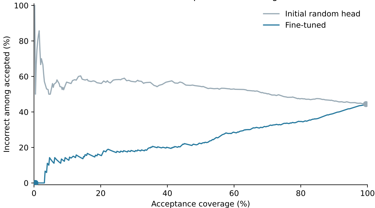
CriticLeanBench: descriptive risk-coverage curves
