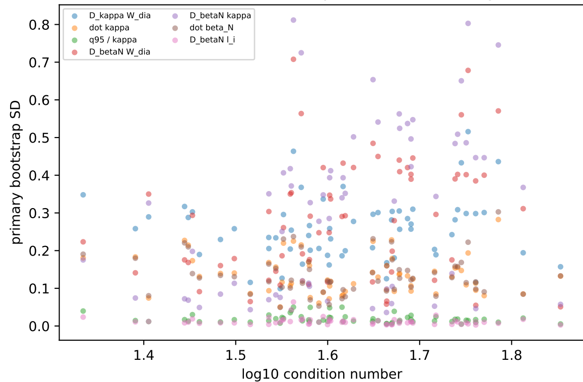
Coefficient uncertainty versus conditioning
