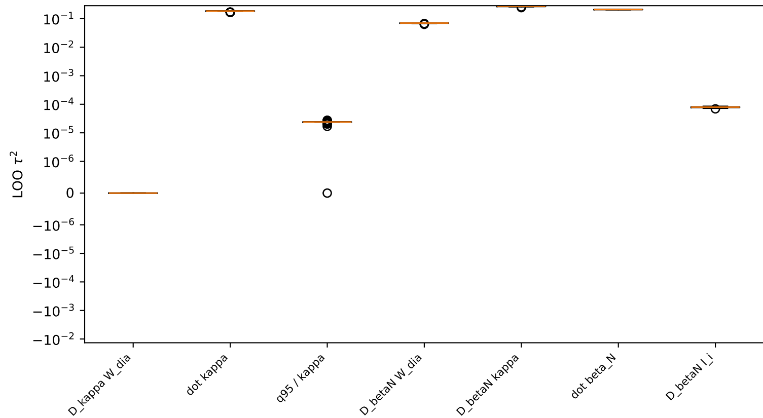
Leave-one-discharge-out \tau^2 sensitivity
