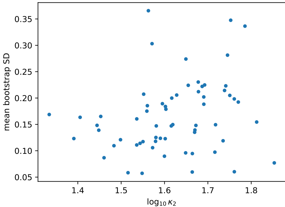
Coefficient uncertainty vs conditioning
