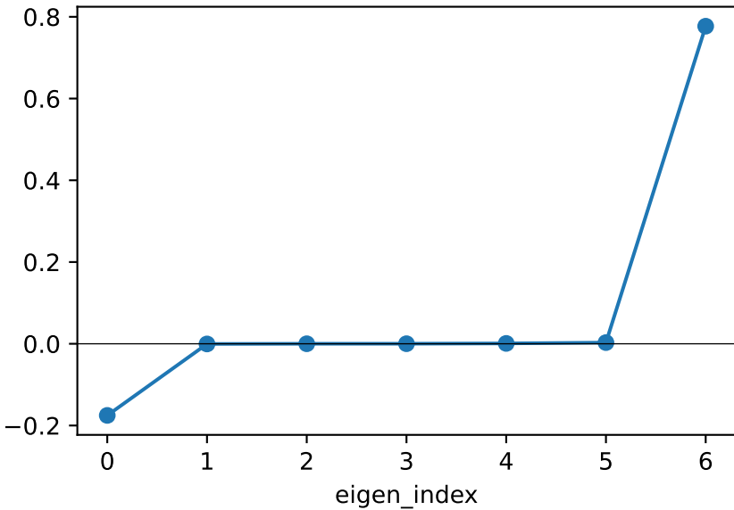
Difference-covariance eigenvalues
