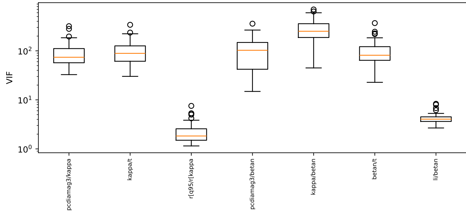
VIF distributions by feature
