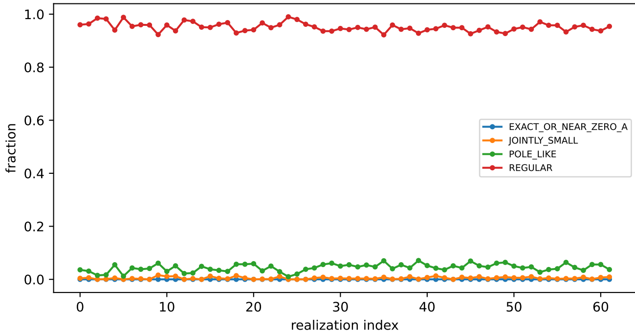
Local degeneracy classification (a_rel=b_rel=0.1)
