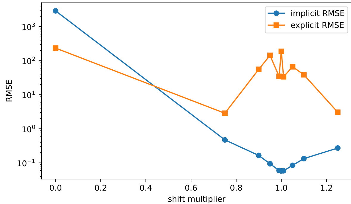
Shift sensitivity (frozen coefficients)
