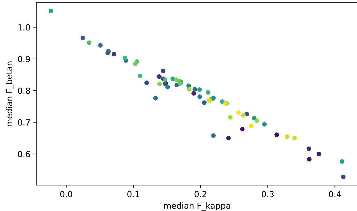
Target-feedback decomposition
