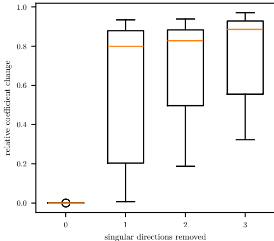
Coefficient movement
