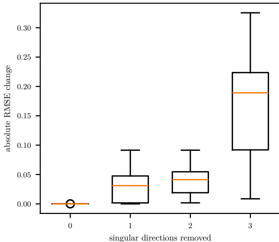
Reconstruction change
