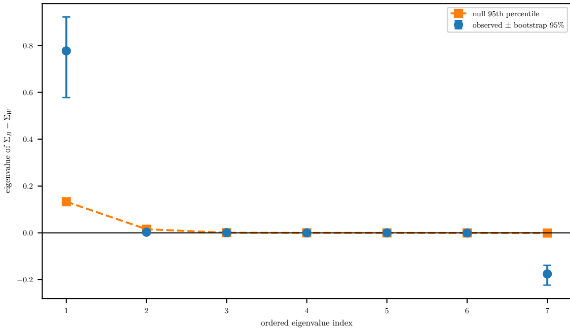
Multivariate eigenvalue uncertainty
